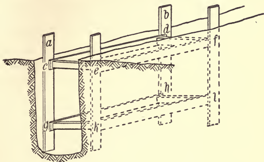
FIG. 13.—SKELETON SHEATHING.
